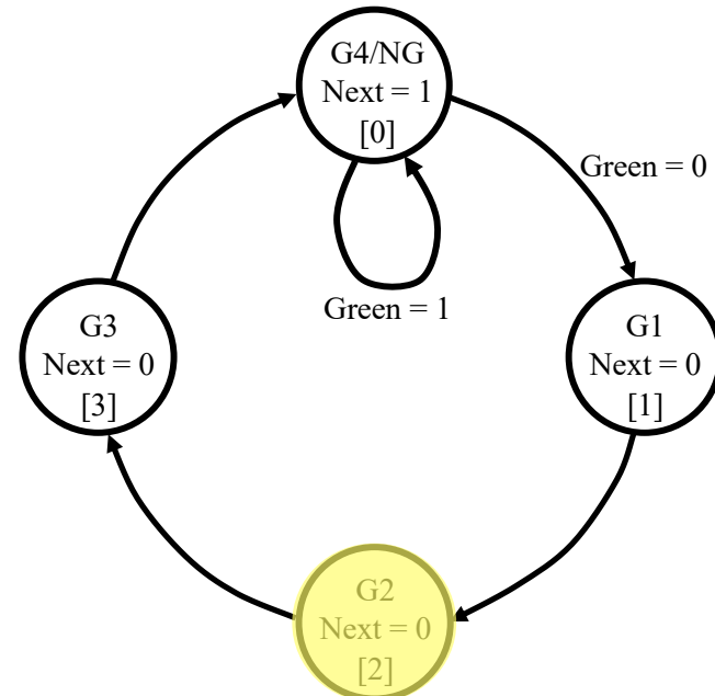
Timer FSM
